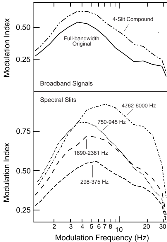
Figure 3. The modulation spectrum (amplitude component) associated with each 1/3-octave slit, as computed for all 130 sentences presented in Experiment 1 [bottom panel]. The peak of the spectrum (in all but the highest channel) lies between 4 and 6 Hz. Its magnitude is considerably diminished in the lowest frequency slit. Also note the large amount of energy in the higher modulation frequencies associated with the highest frequency channel. The modulation spectra of the 4-slit compound and the original, unfiltered signal are illustrated for comparison [top panel].
