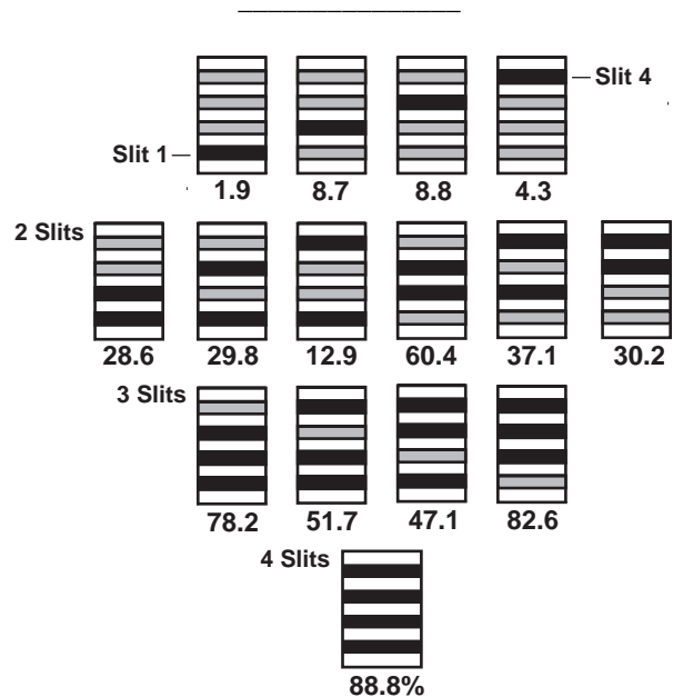
Figure 2. Intelligibility of spectral-slit sentences under 15 separate listening conditions. Baseline word accuracy is 88.8% (4-slit condition). The intelligibility of the multiple-slit signals is far greater than would be predicted on the basis of word accuracy (or error) for individual slits presented alone. The region between 750 and 2400 Hz (slits 2 and 3) provides the most important intelligibility information.
