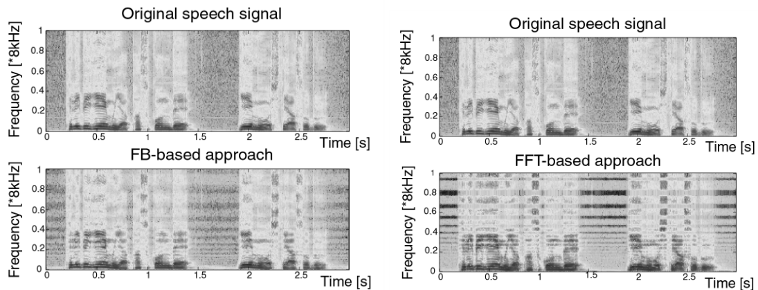
Fig. 1 - Spectrograms of the FB-based (left) and the FFT-based (right) approaches. Top panel: original and bottom panel: processed with compression rate of 50%.
